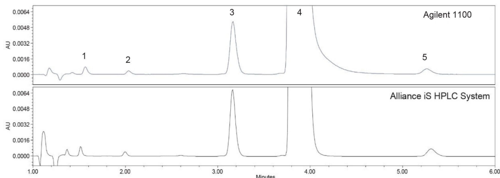
Figure 2. Stacked chromatograms of the sample solution for the ibuprofen organic impurities analysis and used for known and unknown impurities measurements. Peak 1 = Unspecified impurity 1. Peak 2 = Related compound J. Peak 3 = Unspecified impurity 2. Peak 4 = Ibuprofen. Peak 5 = Related compound C.
