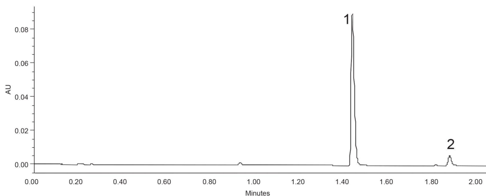
Figure 1. Analysis of ritlecinib on an ACQUITY UPLC H-Class Plus System with a Waters ACQUITY BEH C 18 RP Column with MaxPeak Premier Technology, 3.0 x 50 mm, 1.7 µm. 1) ritlecinib, 2) impurity.
