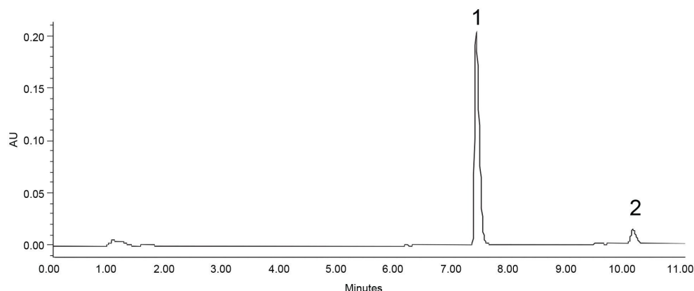
Figure 3. Analysis of ritlecinib using an Agilent 1260 Infinity II System with an XBridge Premier BEH C 18 , 3.0 x 100 mm, 3.5 µm Column. 1) ritlecinib, 2) impurity.
