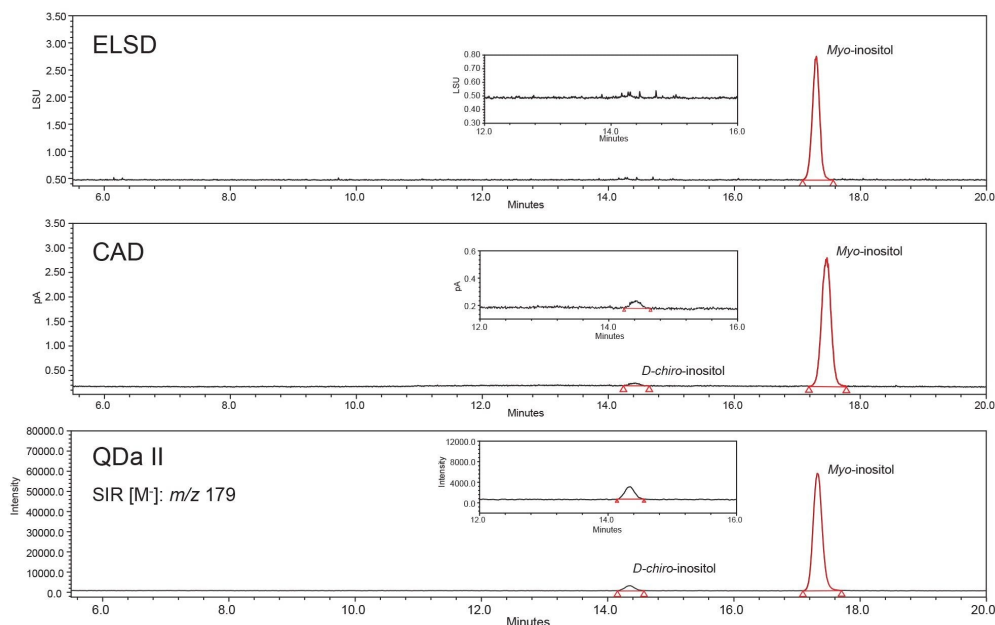
Figure 2. Chromatograms of a dietary supplement sample (DS D) acquired by the Waters ELSD, CAD, and ACQUITY QDa II Mass Detector. Expanded views are included to highlight the D-chiro-inositol peak. Sample concentrations were approximately 200 \mu\text{g/mL} for the ELSD and CAD chromatograms and 4 \mu\text{g/mL} for the ACQUITY QDa II Mass Detector chromatogram.
