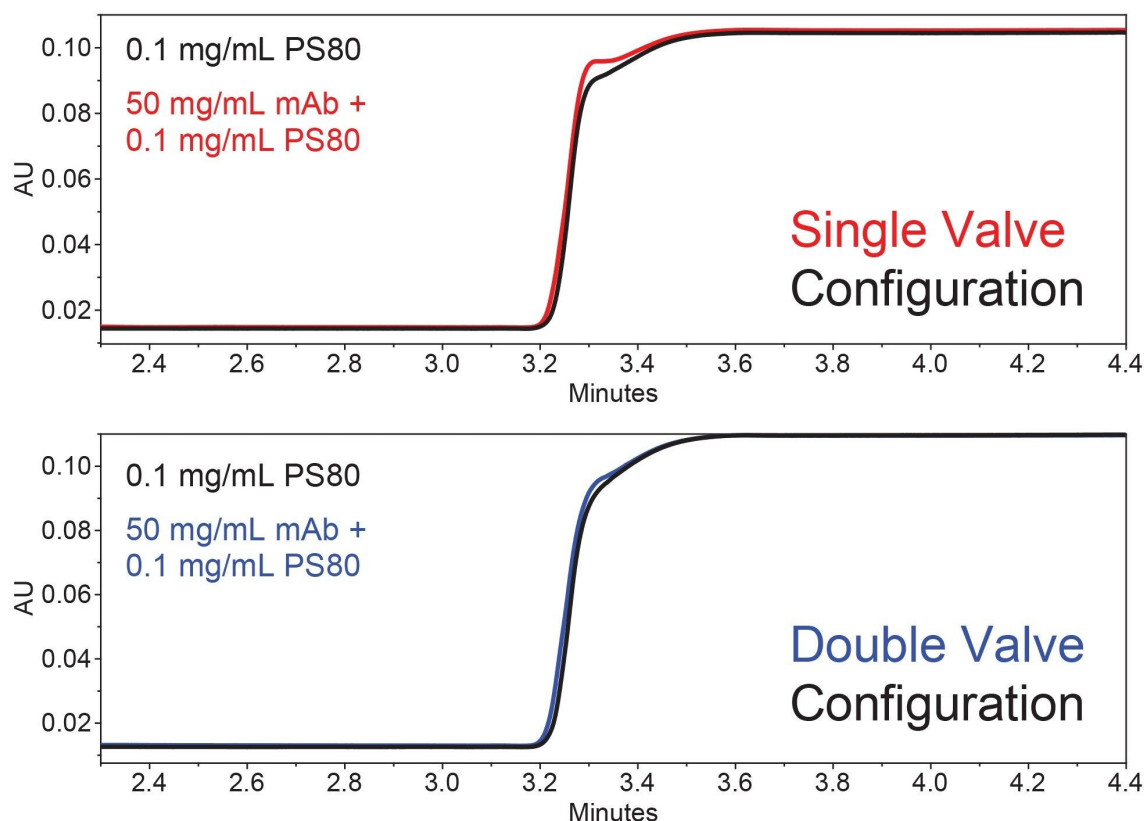
Figure 2. UV chromatograms comparing 0.1 mg/mL PS80 standard and 50 mg/mL mAb-spiked sample with 0.1 mg/mL PS80 for both valve configurations.
