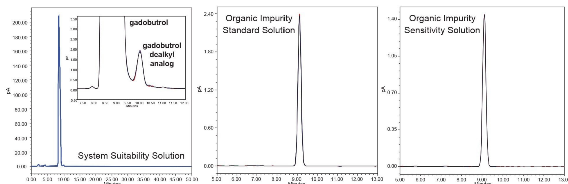
Figure 5. System suitability results for gadobutrol organic impurity method and overlaid CAD chromatograms for the system suitability mixture ( n = 3 ), standard solution ( n = 6 ) and sensitivity solution ( n = 6 ) which are prepared at 10 mg/mL, 0.005 mg/mL, and 0.003 mg/mL respectively.
