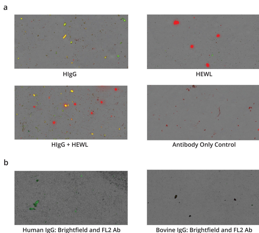
Figure 2. Combined brightfield and fluorescence images from the Aura System from solution phase antibody labeled HIgG, HEWL, and HIgG + HEWL mixed sample (a) and solution phase labeled HIgG and Bovine IgG (b).
