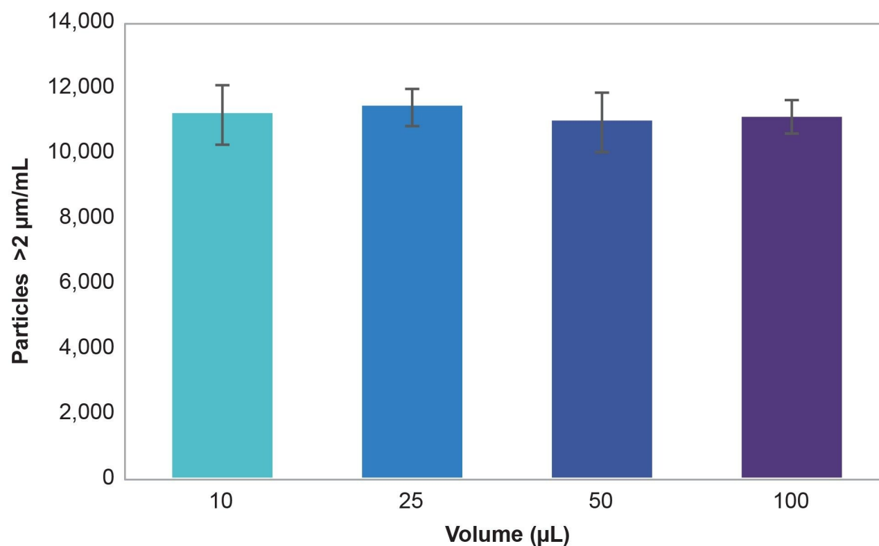
Figure 2: Impact of volume on polydisperse samples in BMI. Varying volumes of ETFE samples were measured. Particle counts were all within 4% of each other, demonstrating sample volume did not impact measurement precision.
