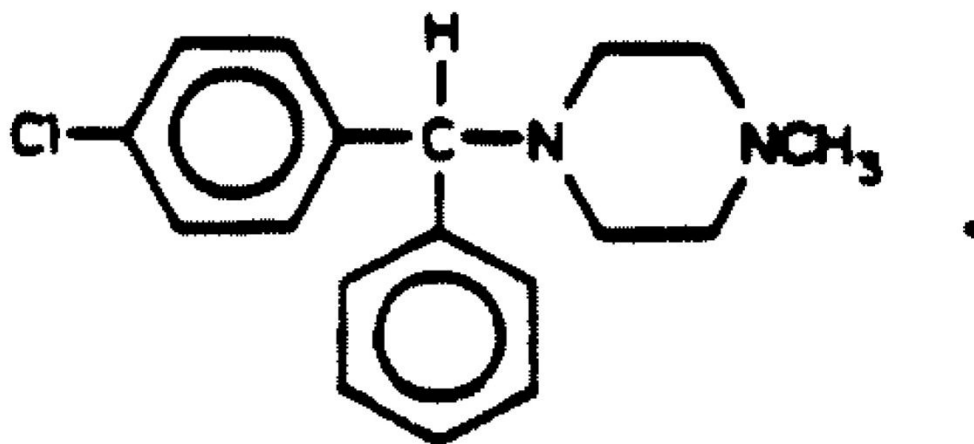
2. Chlorcyclizine HCL
