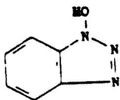
1. 1-hydroxybenzotriazole (IS)
